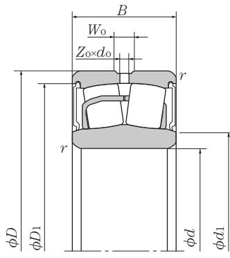
Cylindrical bore
