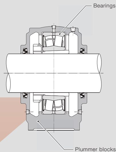
Pulley bearing in contaminated environment
