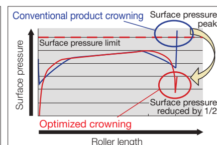
Optimized crowning is utilized on the rolling elements
