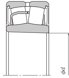
Tapered bore
