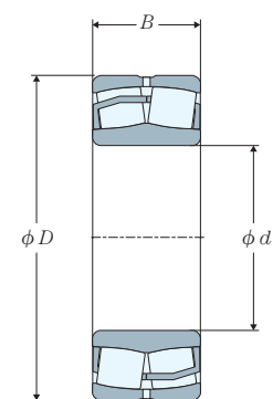
Cylindrical bore (Type EA)
